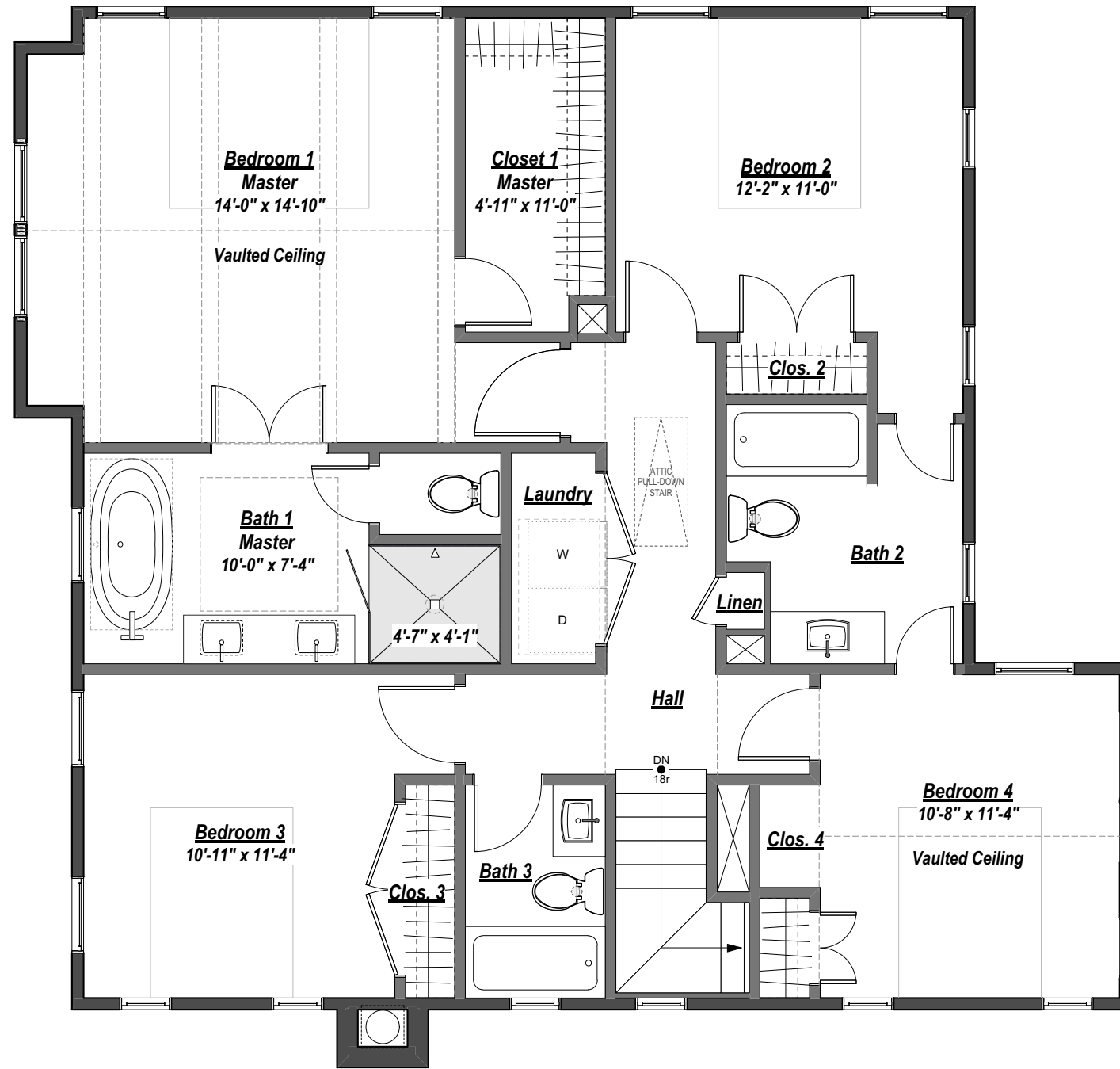
#708 Belt Loop - Plan 4a: Level 2
