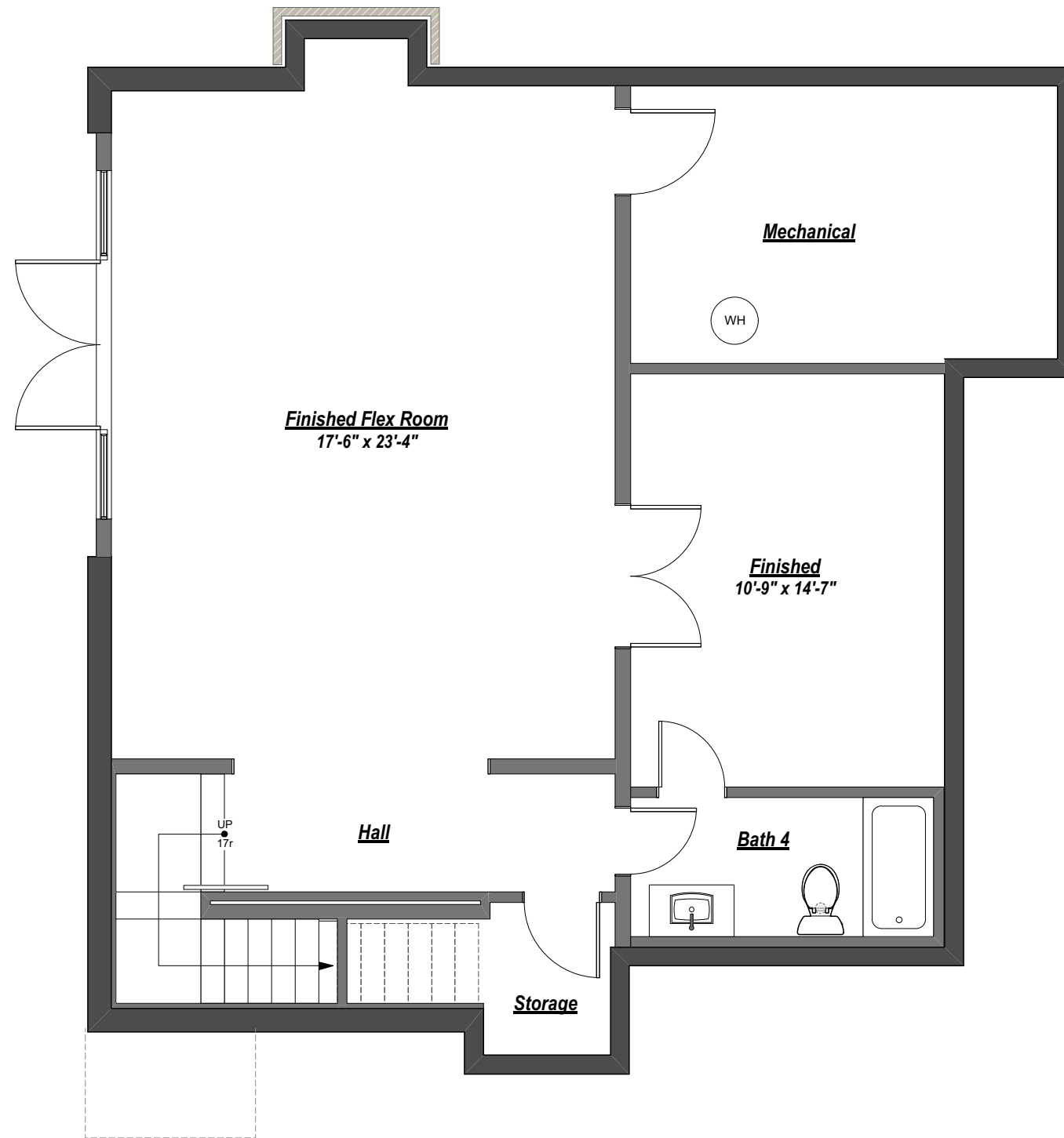
#744 Belt Loop - Plan 1b: Basement
