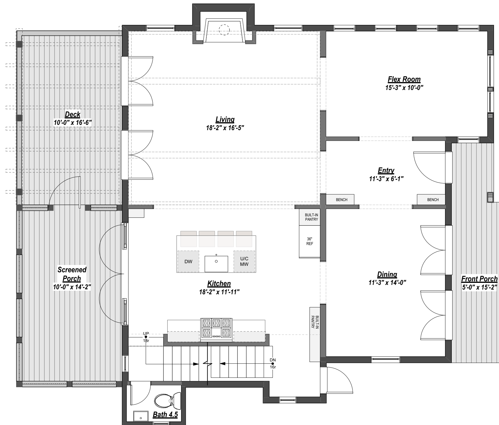
#744 Belt Loop - Plan 1b: Level 1
